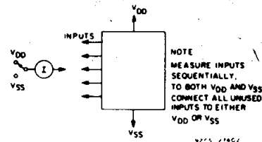
Fig. 19 — Input current test circuit.
